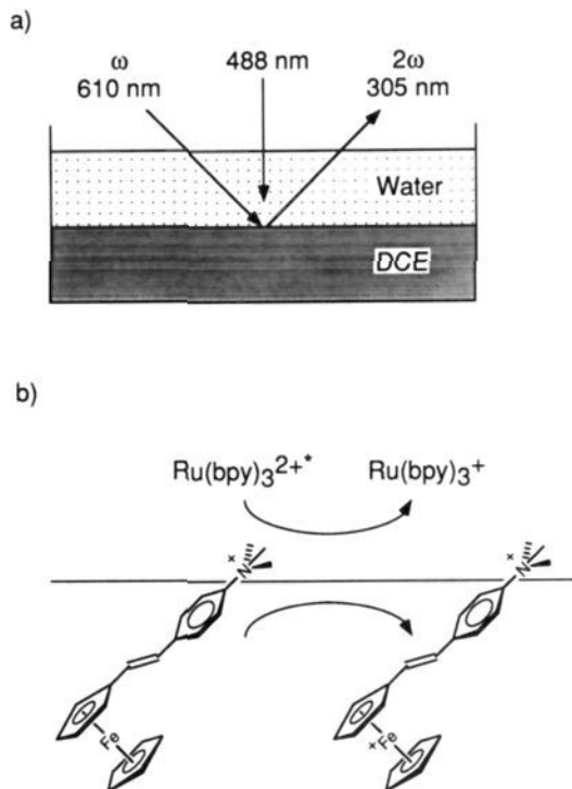
Figure 1. (a) Surface SHG experiment for monitoring the photoinduced electron-transfer reaction from 1^+ to \text{Ru}(\text{bpy})_3^{2+*} at the water/DCE interface. (b) Schematic representation of the photoinduced electron-transfer reaction at the water/DCE interface.
